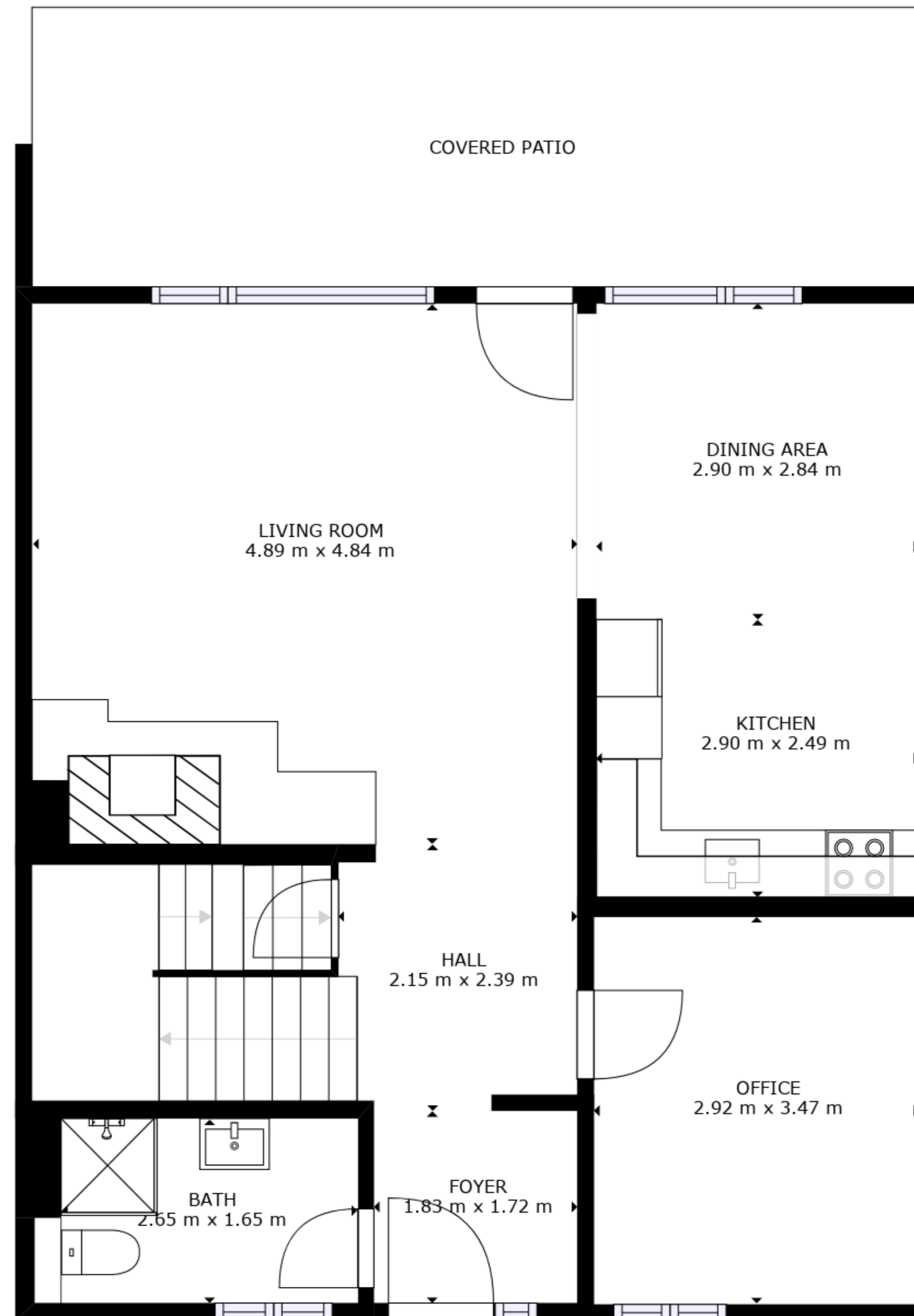
FLOOR 2
