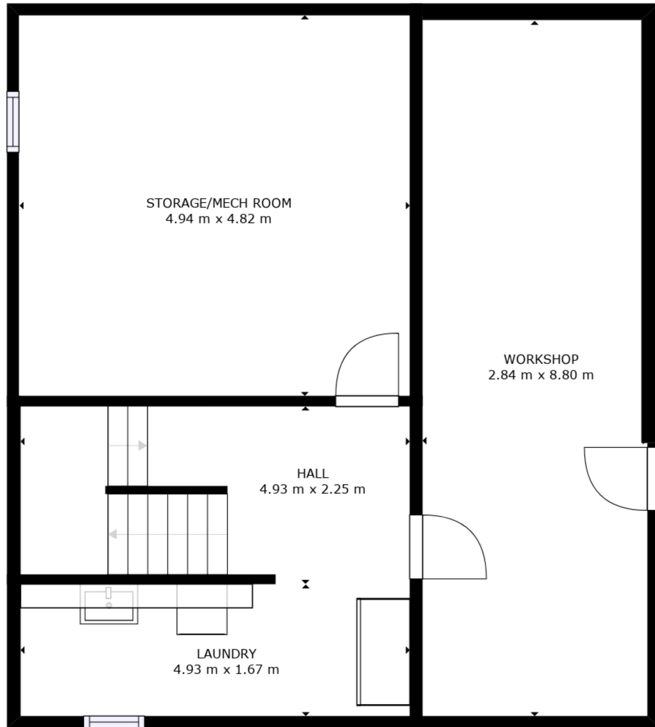
FLOOR 1
